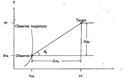
Fig. 1. Geometry of bearings-only localization problem.
