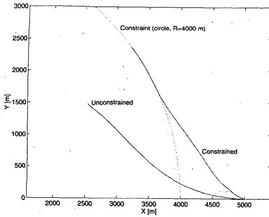
Fig. 6. DI example. Dotted line represents constraint.
