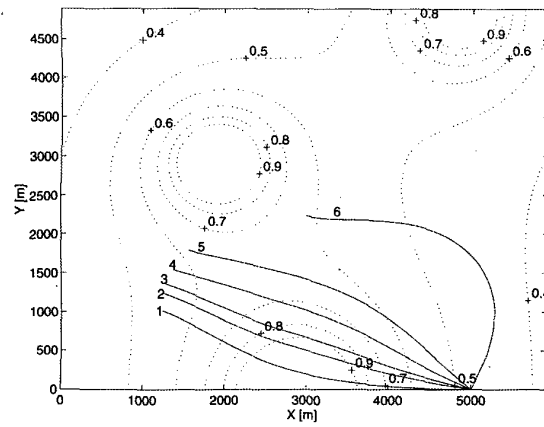
Fig. 8. Optimal trajectories in presence of threat.
