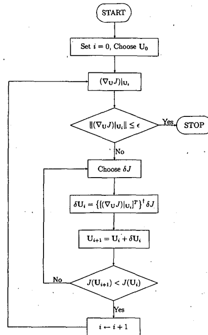
Fig. 2. Direct optimization procedure.
